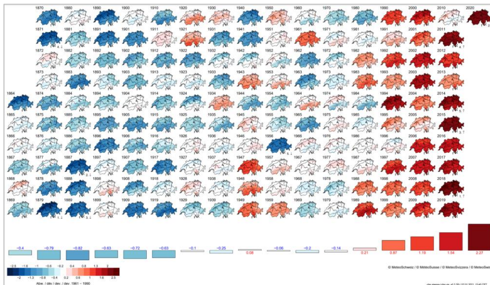
Figure 82 Temperature evolution from 1864 to 2020. Source: OFMC (2020).
