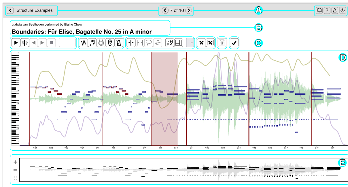
Figure 4.1: The main CosmoNote interface showing an annotated excerpt of Beethoven’s Für Elise . The cyan rectangles highlight the different elements: (A) Navigation bar for the collection and account options; (B) Names of the piece, performer, composer; (C) Audio controls, annotation types, and other control buttons; (D) Visualization pane – annotations are displayed in shades of red on top of the waveform (pale green), piano roll (shades of blue), loudness (mauve), tempo (olive), and harmonic tension (shades of brown, not shown); and, (E) Contextual zoom.
