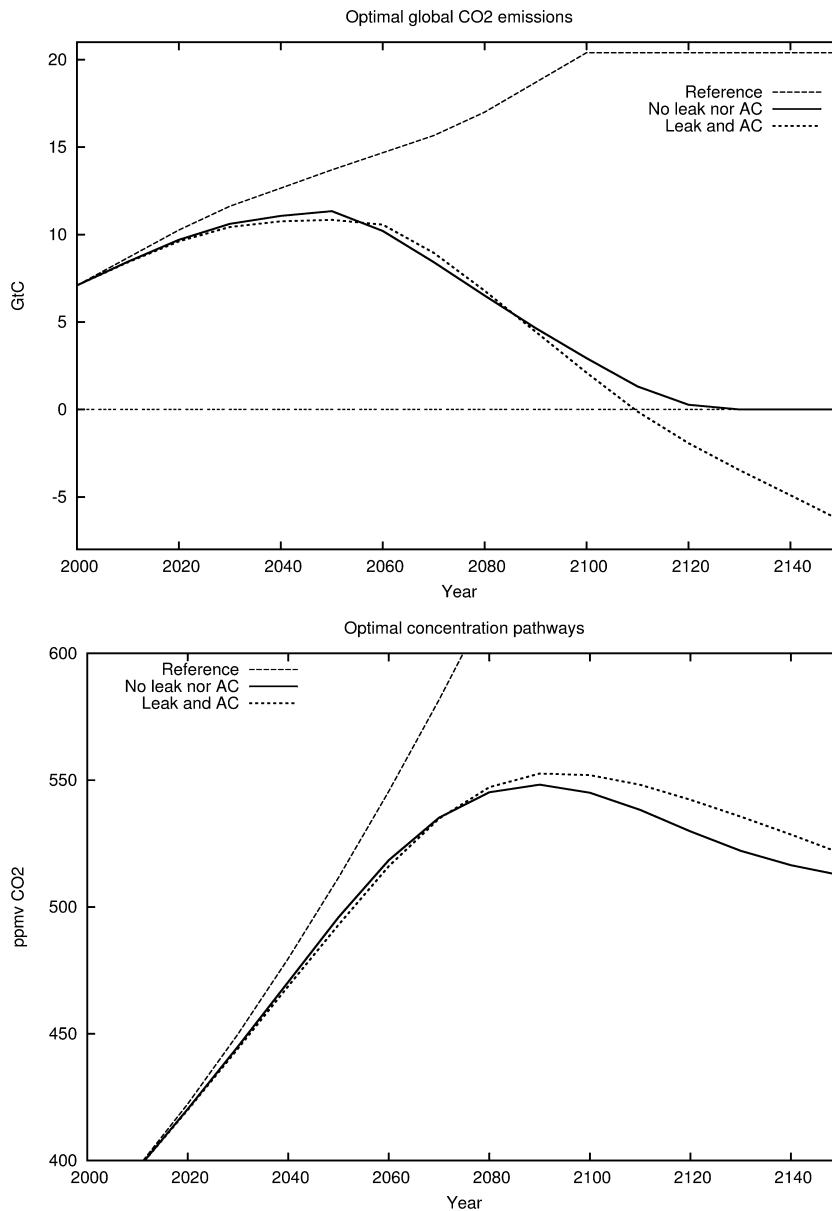
Fig. 2. Optimal CO 2 trajectories. Upper panel , global carbon emissions, not including emissions from leaks due to underground storage. Lower panel , atmospheric CO 2 concentration in parts per million
