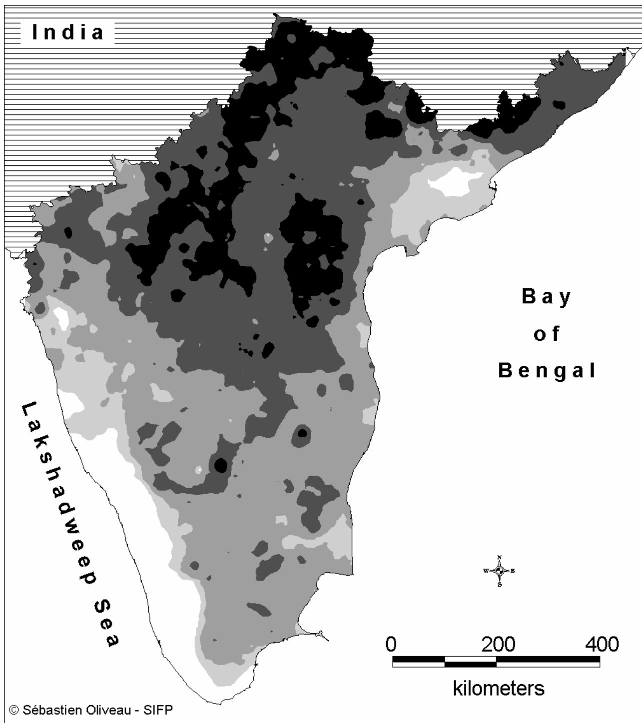
Figure 8: Smoothed gender index of literacy in South India, 1991
