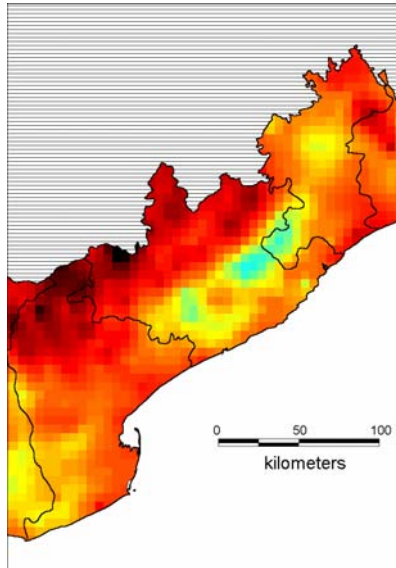
Figure 3: Smoothed fertility values obtained by kriging (villages in three districts of Northeast Andhra Pradesh)
