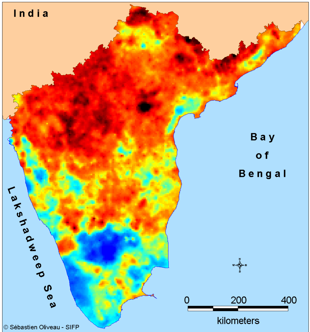
Figure 6: Smoothed fertility (CWR) estimates in South India, 1991.
