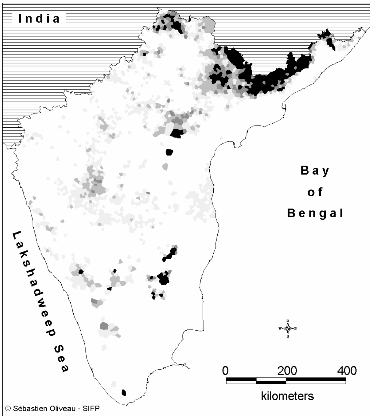
Figure 9: Smoothed tribal share in South India, 1991
