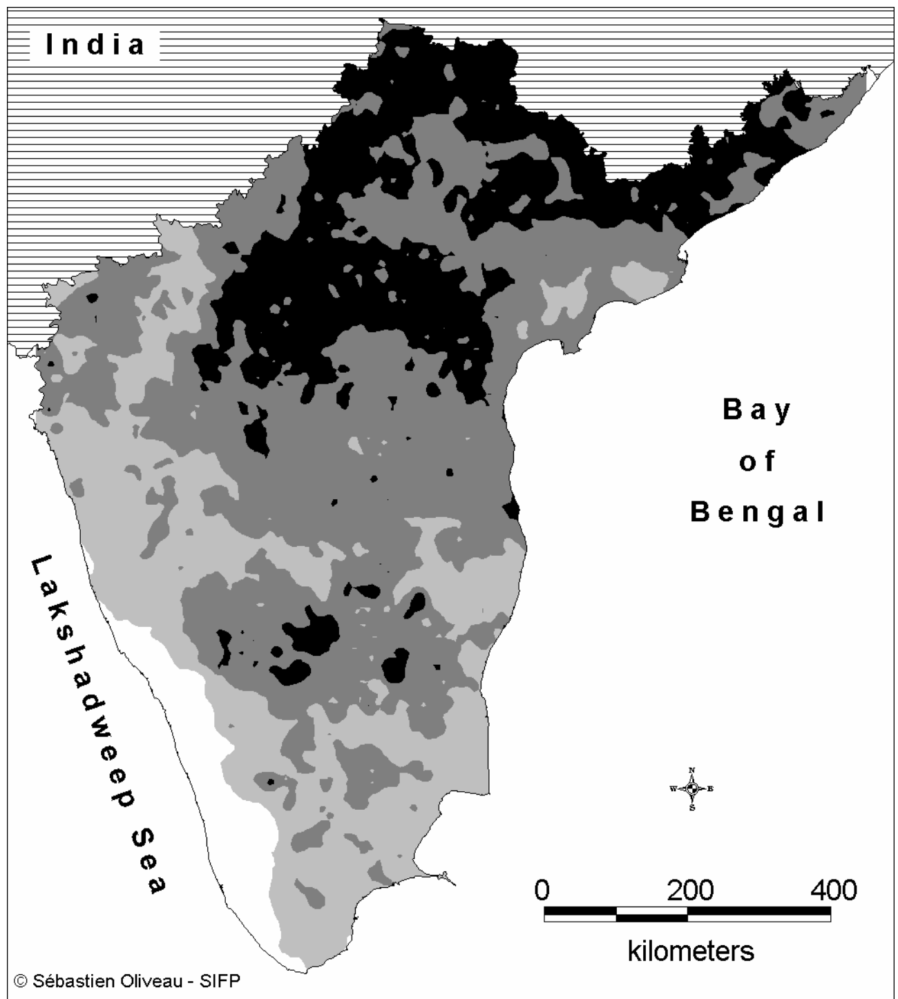
Figure 7: Smoothed literacy estimates in South India, 1991
