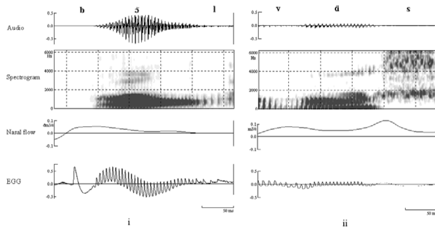
Figure 5. Data illustrating the criteria used for characterizing carryover. (i) synchronous offset of NAF, in the word “bon” [bõ] 'good'. (ii) carryover in “Provence”[pɔvãs]. Data taken from spontaneous speech.
