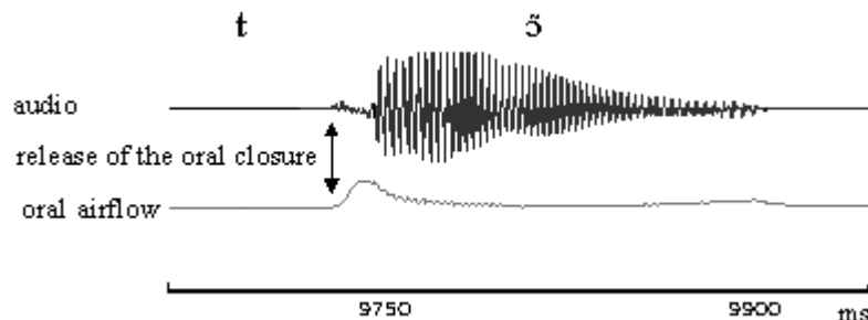
Figure 2. Waveform and aerodynamic data for the word “ton” [tɔ̃] ‘your’. The two arrows show that the stop burst is well aligned with the increase of oral airflow. (Data collected with PCquiner).
