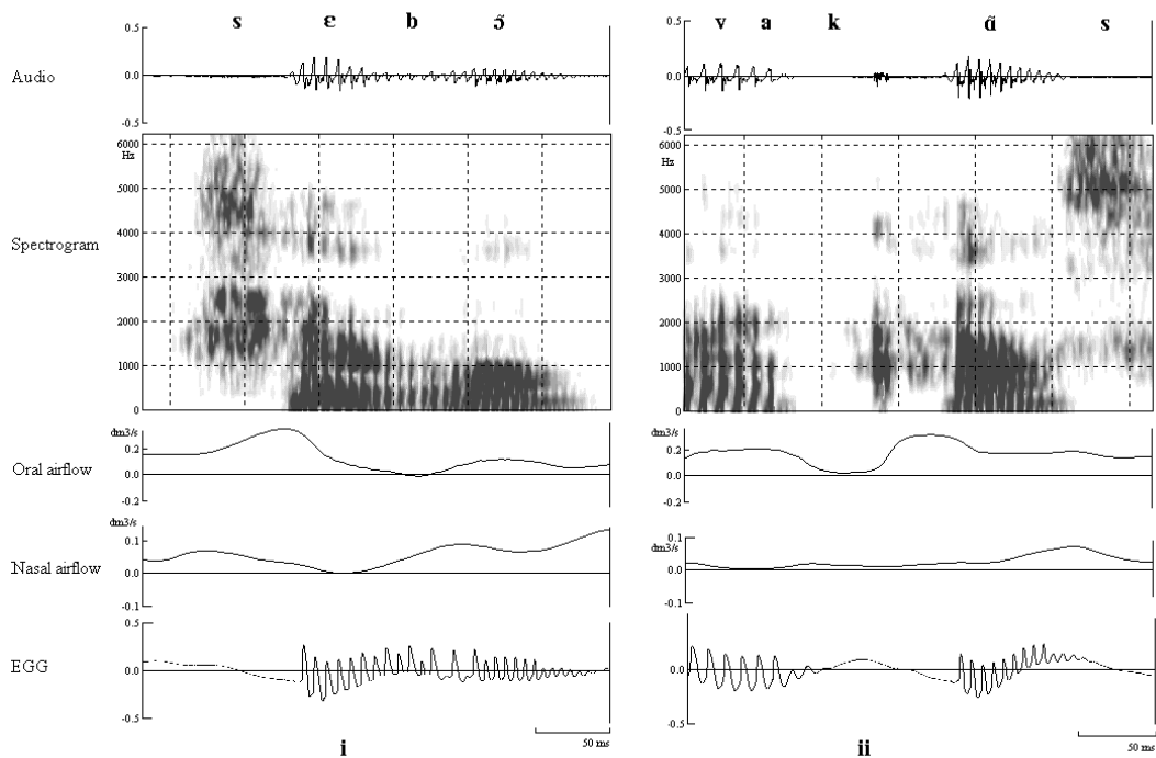
Figure 6. Examples of anticipatory nasal airflow. (i) “C’est bon” [se bɔ̃] ‘is it all right’. (ii) “vacances” [vakɑ̃s] ‘holidays’ (spontaneous speech)
