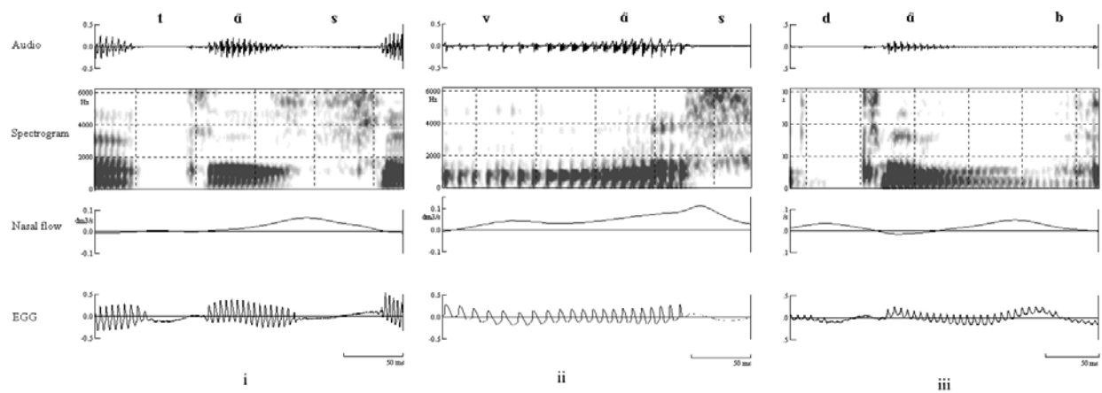
Figure 4. Data illustrating the criteria used for characterizing anticipation. (i) synchronous onset of NAF, in the word “attention” [atãsjs] 'be careful'. (ii) anticipation in “Provence”[pɔvãs]. (iii) delay in “d’embouts” [dãbu] ‘nozzles’. Data taken from spontaneous speech.
