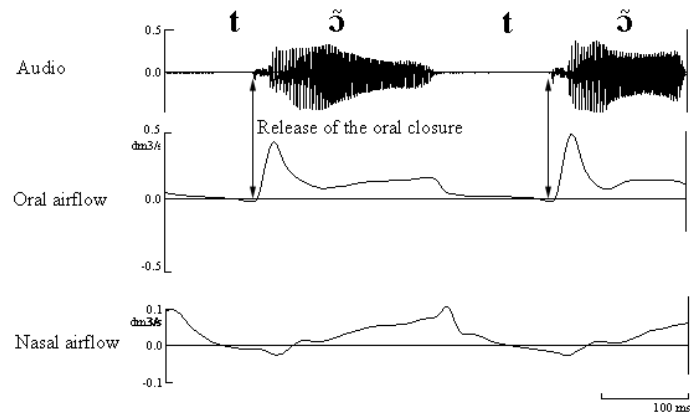
Figure 1. Waveform and aerodynamic data of the word “ton” [tɔ̃] ‘your’. The arrows show that the stop burst is well aligned with the increasing of oral airflow. (Data collected with Eva workstation).
