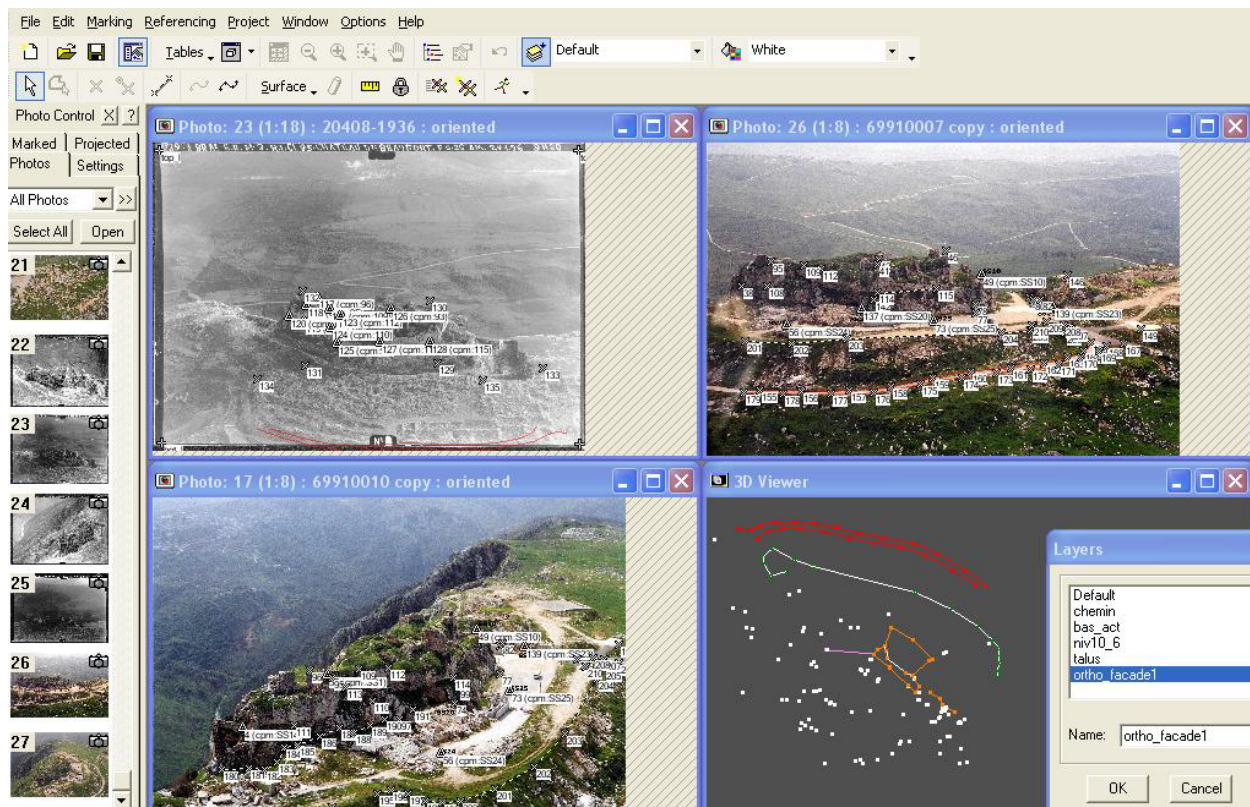
Figure 8. Multi-image restitution within PhotoModeler 5.0
