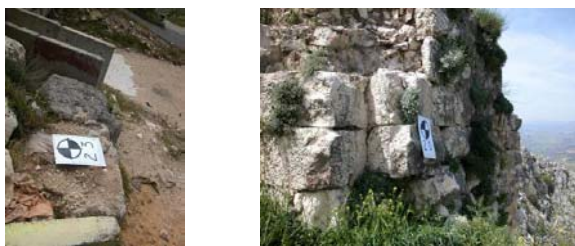
Figure 4. Examples of targets used for the reference points
