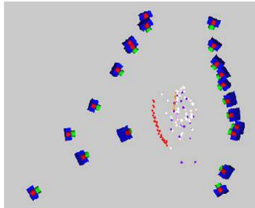
Figure 7a. Overview of the camera stations and the block configuration after the exterior orientation
