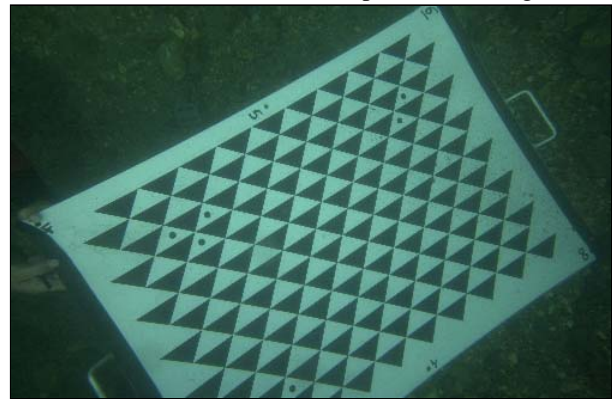
Fig. 3. Photograph for calibration process with Photomodeler. Calibration grig lend by Comex.
