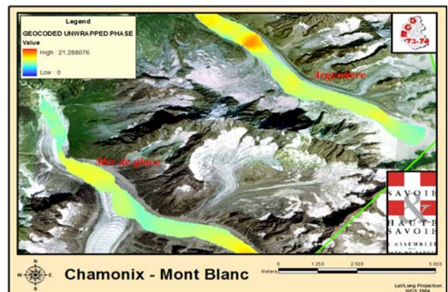
Figure 2. Mer-de-Glace and Argentière glacier 1-day displacement measured from ERS tandem data, March 96.
