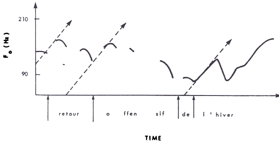
Fig. XVI-23. Use of the F_0 contour to divide a sense group into words. Dashed lines indicate initial rise associated with each lexical word.
