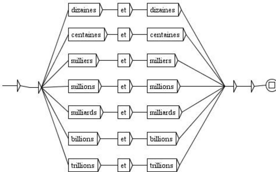
Fig. 3. Excerpt of a local grammar of French determiners.
