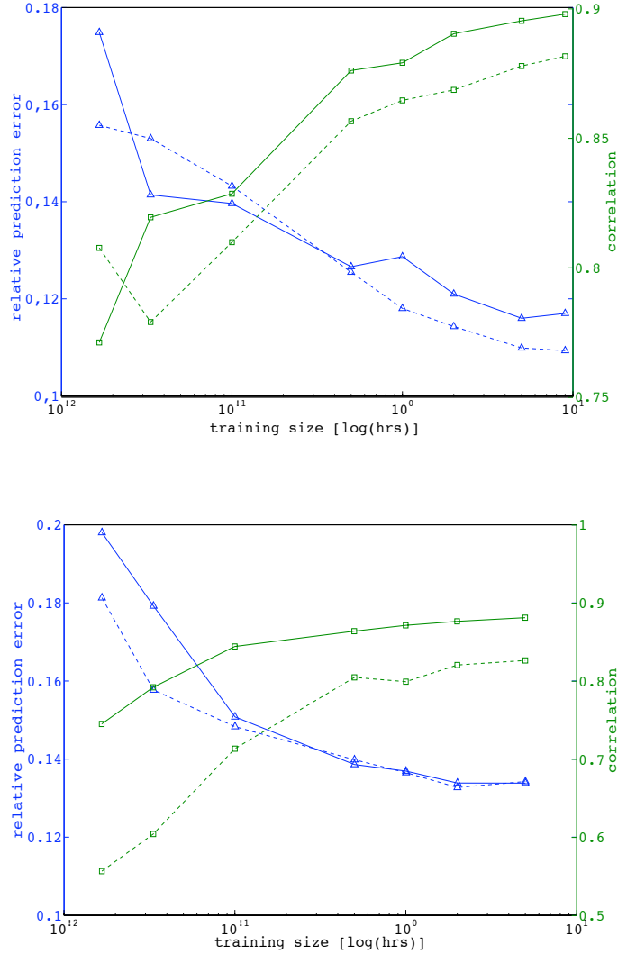
FIG. 1 – Performance as a function of the training set size. Top : laboratory speech. Bottom : acted speech. Baseline model is represented with dash-lines. Proposed model is represented with plain-lines. Relative prediction errors are plotted with triangles and correlation score with squares.
