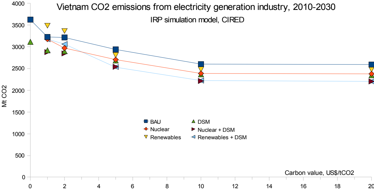
Figure 2. Assessment of the results of the CO 2 emissions mitigation potential using various scenarios of development for Vietnam’s power sector in the 2010-2030 period.
