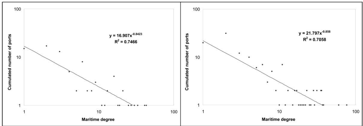
Figure 3. Scale-free structure of the Northeast Asian liner network (1996-2006)
