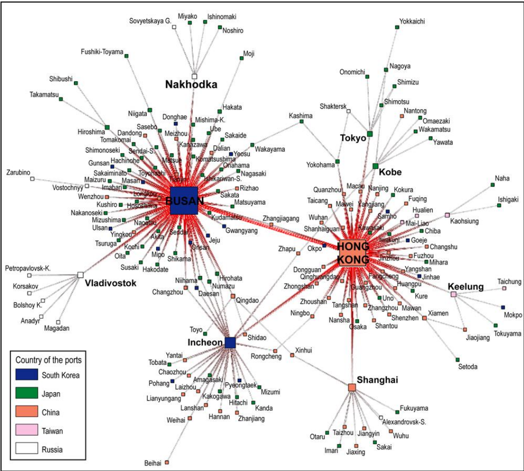
Figure 5: Graph of dominant flow structure (2006)
