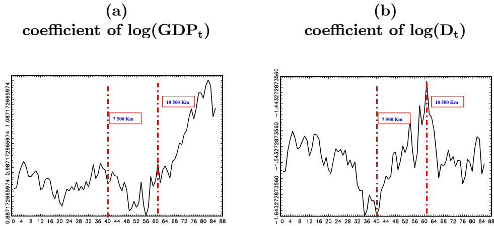
Figure 5. Paths of the FLS coefficients of the import equation for \mu = 1
