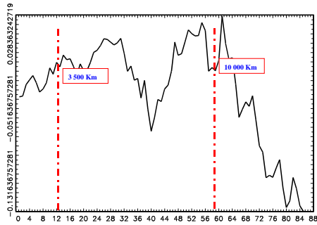
Figure 3. Residual efficiency frontier for the export equation
