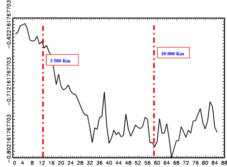
(b) coefficient of \log(D_t)
