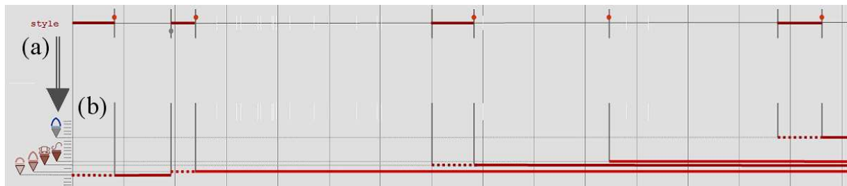
Figure. 5. (a) - activity indicator for feature “style”– when selected by the user opens (b) - feature readout (here stylistic affiliations represented by icons – Romanesque, Gothic, Renaissance, Baroque and neoGothic elements successively appear during the evolution of the artefact). Thick lines on the activity indicator identify periods when the feature appears. The continuous lines in the feature readout indicate the feature persists in time (note here that the bottom line – Romanesque stylistic affiliation – ends with the appearance of gothic elements, a visual indication that the initial structure is not complemented but replaced).
