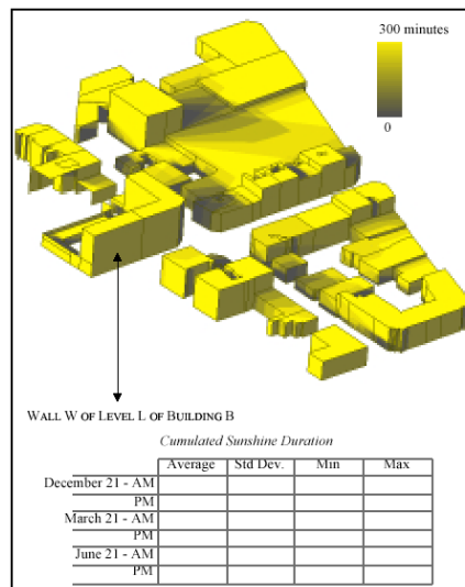
Figure 6. Integrating solar computation within the GIS, as numerical data and simulation textures
