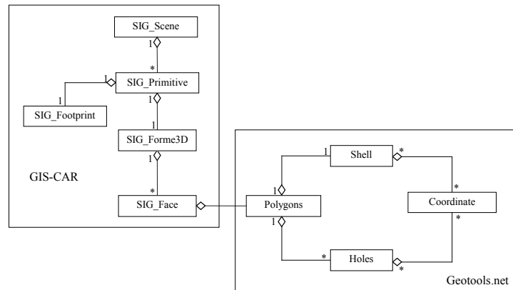
Figure 5. Architectural primitives used in order to describe a building
