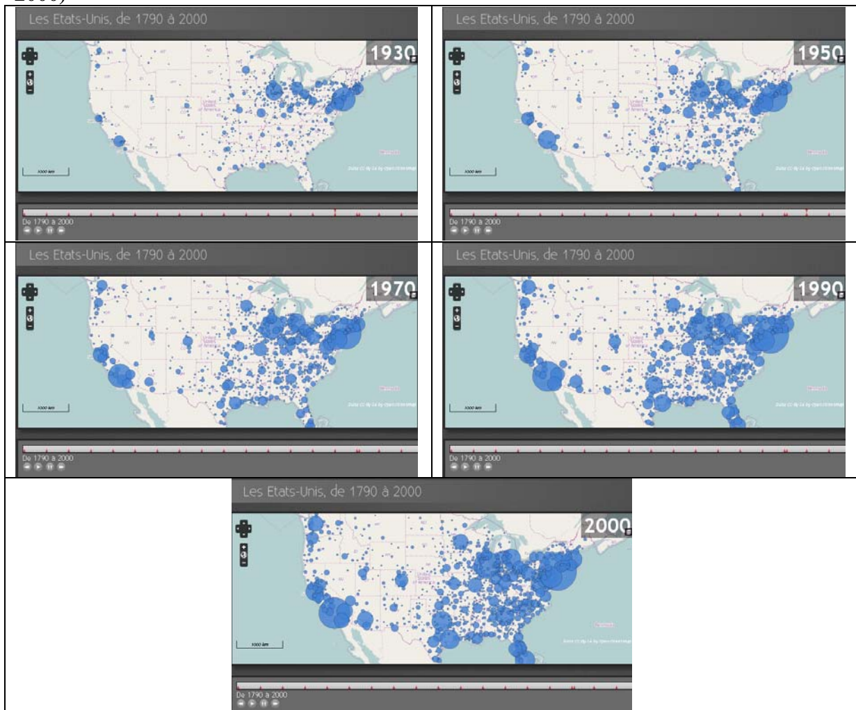
Figure 9: Step by step animation of the urban populations in US (selected dates, 1930-2000)
