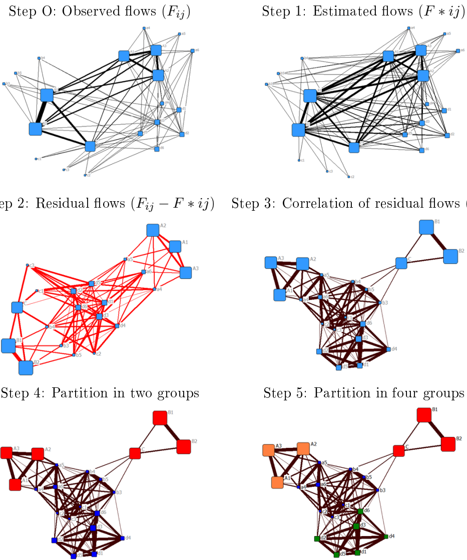
Figure 1: Application of the MaxCor algorithm on a theoretical example
