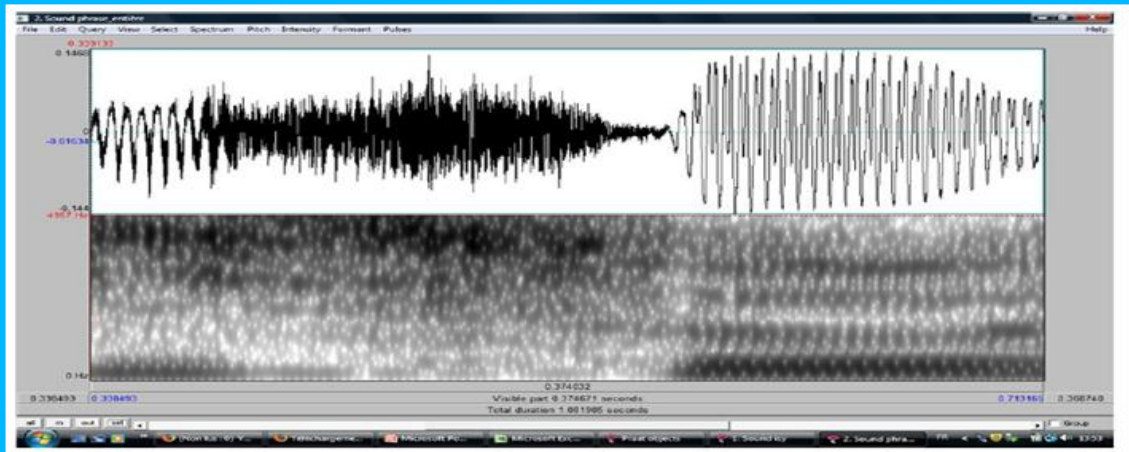
Figure 5. The acoustic signal and spectrogram for the [isø] sequence. The inferior limit of the frication noise slightly decreases from vowel [i] to vowel [ø].
