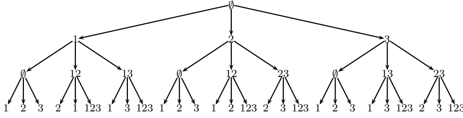
Fig. 3 Set of scenarios \mathfrak{S}(\mathbf{U}^{M,\infty}, 3)
