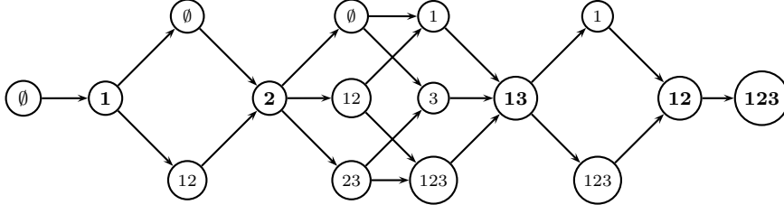
Fig. 2 Scenario \mathcal{S} completed for computing the Shapley II value. Boldface figures indicate nodes of the scenario
