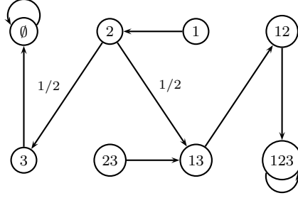
Fig. 1 The digraph \Gamma of the Confucius process
