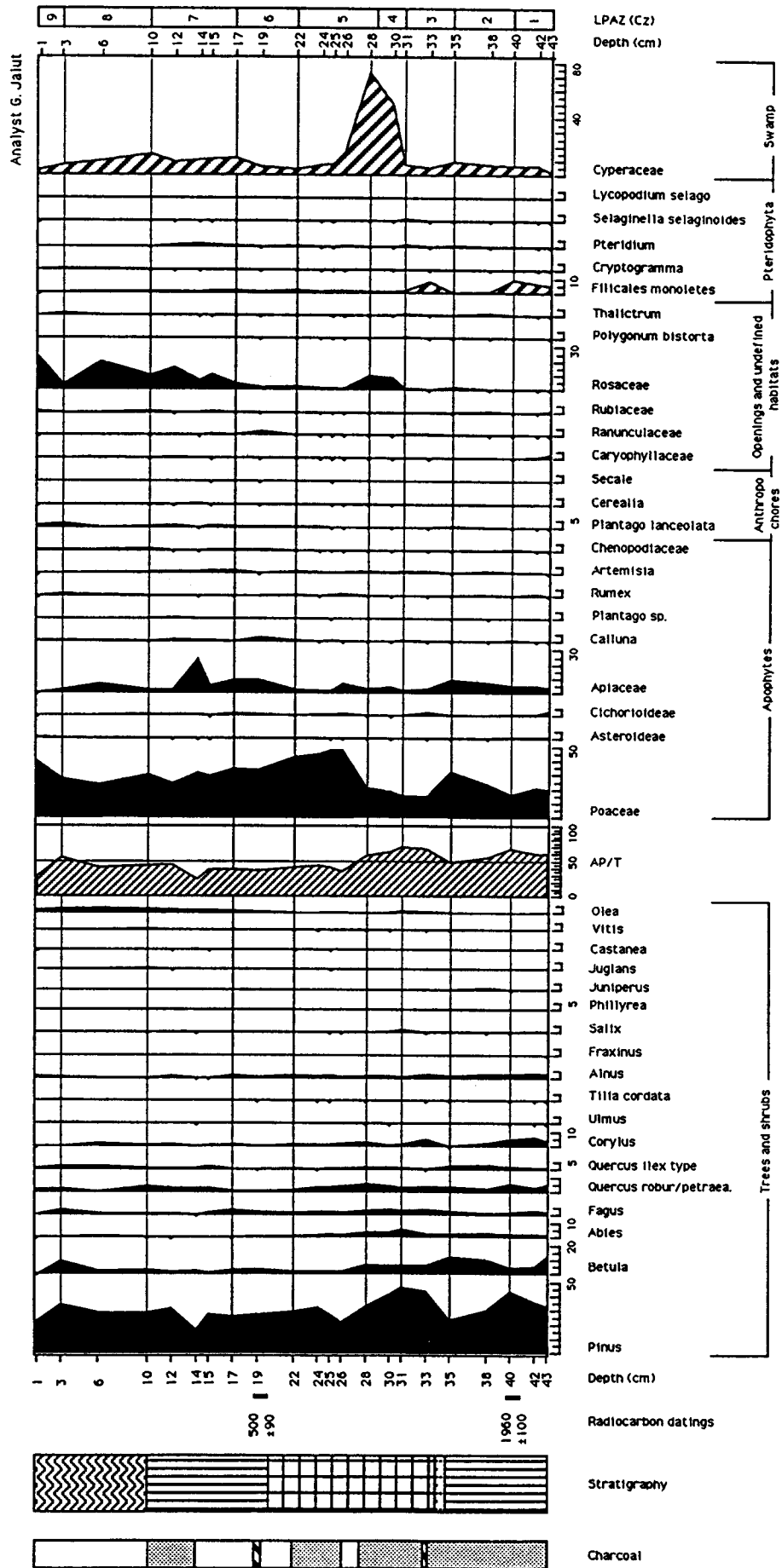
Fig. 5. Pollen diagram from Pla de Croutz
