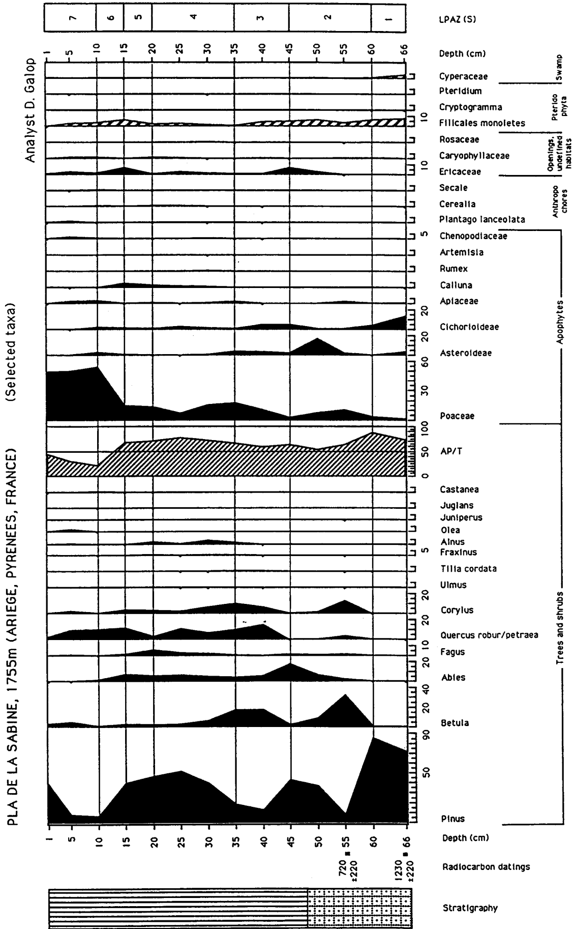
Fig. 8. Pollen diagram from Pla de la Sabine
