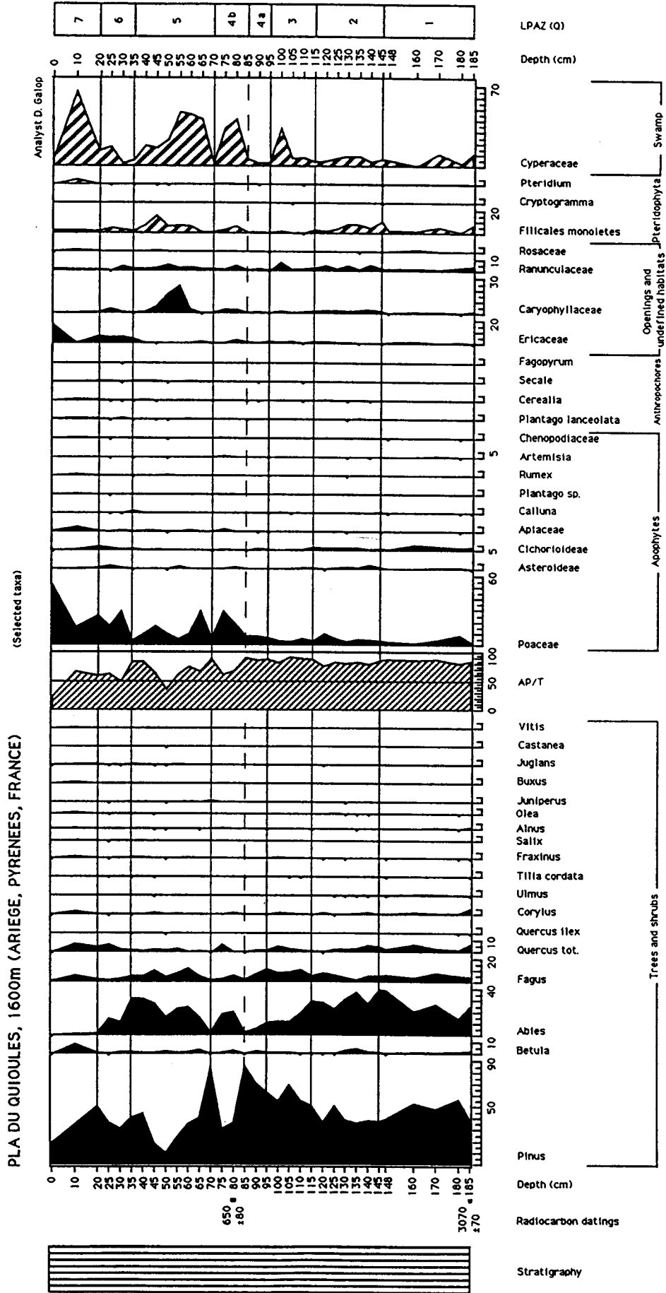
Fig. 7. Pollen diagram from Pla de Quioules
