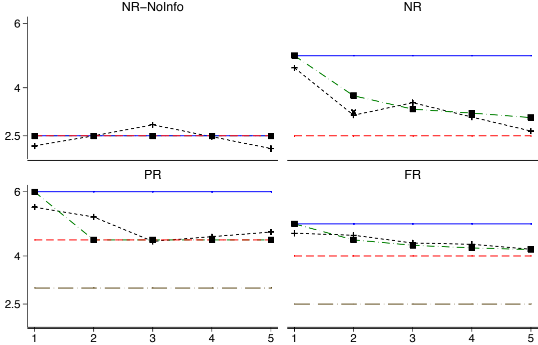
Legend. - - - Mean empirical value \hat{v}_n -■- Theoretical value v_n ; - - v_1 ; - - \text{cav } u ; - - u Note. For each game, the figures plot the mean empirical value, the theoretical value and the lower and upper bounds of the value functions for each length n \in \{1, \dots, 5\} in abscissa. For the NR game with n = 2 stages, we also plot the average value observed in Feltovich (2000) (appears as a \times ).
