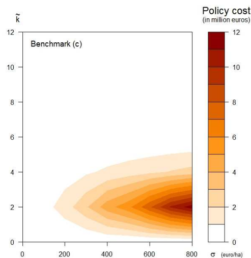
Figure 5: Policy cost for different combinations of (\sigma, \tilde{k}) from benchmark (c)
