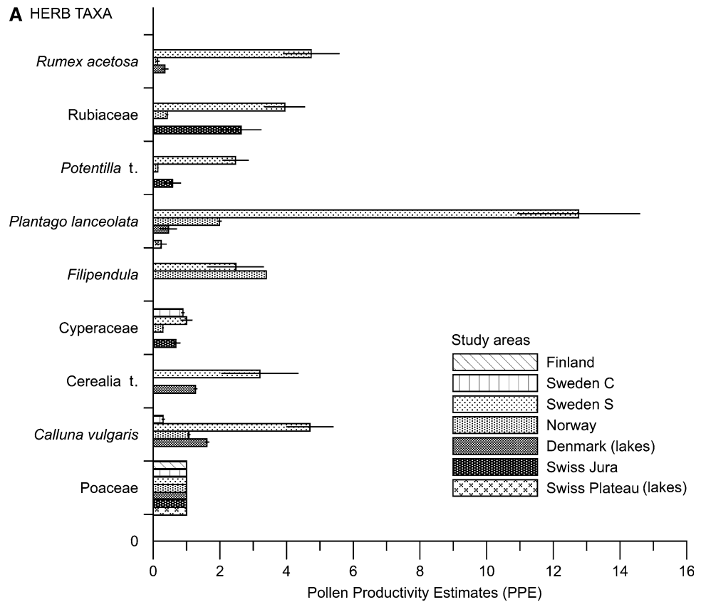
Fig. 4 Pollen productivity estimates with error estimates for major taxa
