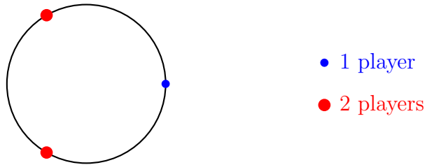
Figure 4: Worst equilibrium \tilde{x}^\perp on C with 5 players.
