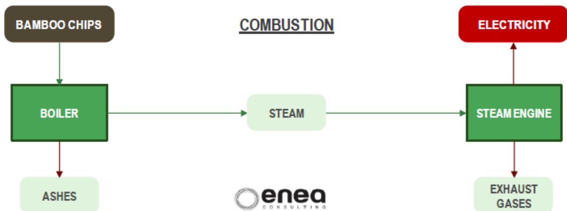
Figure 3. A diagram of combustion process from bamboo biomass to electricity (Kerlero de Rosbo and de Bussy, 2012)
