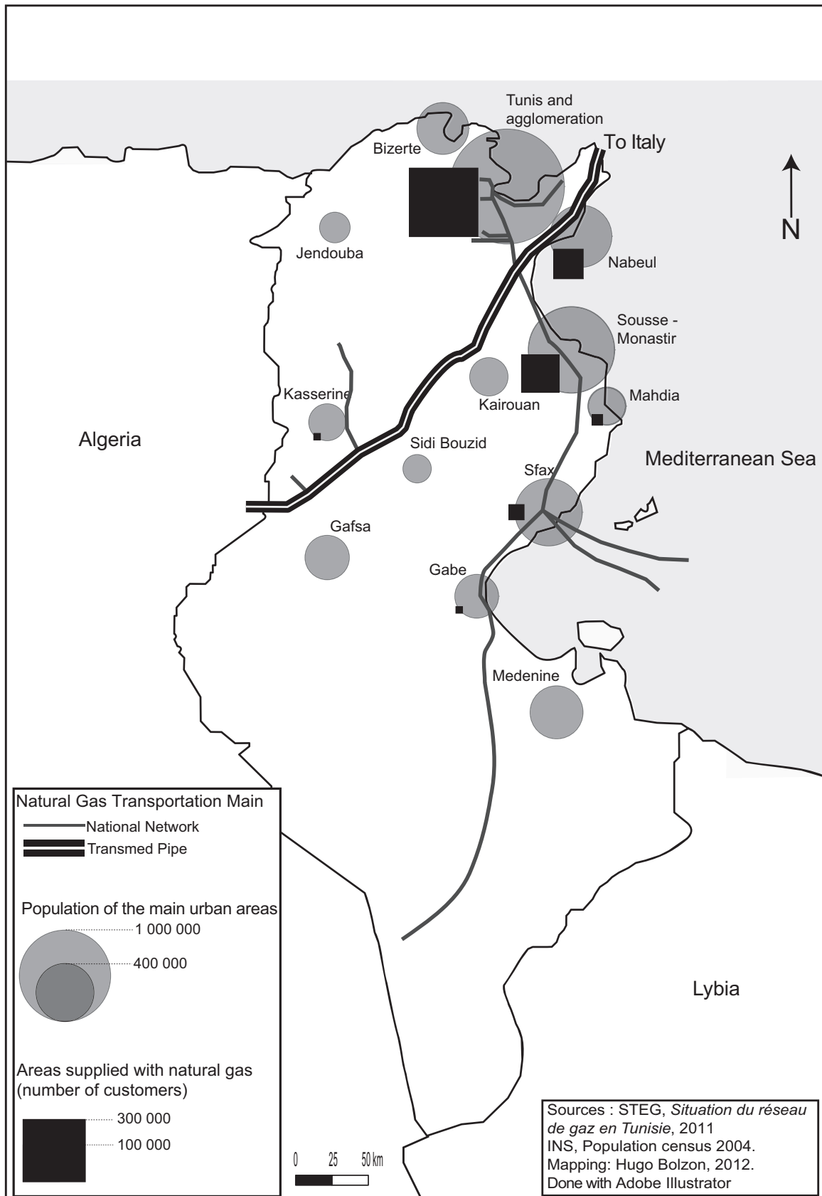
Fig. 1. Tunisia natural gas network and main supplied areas.
