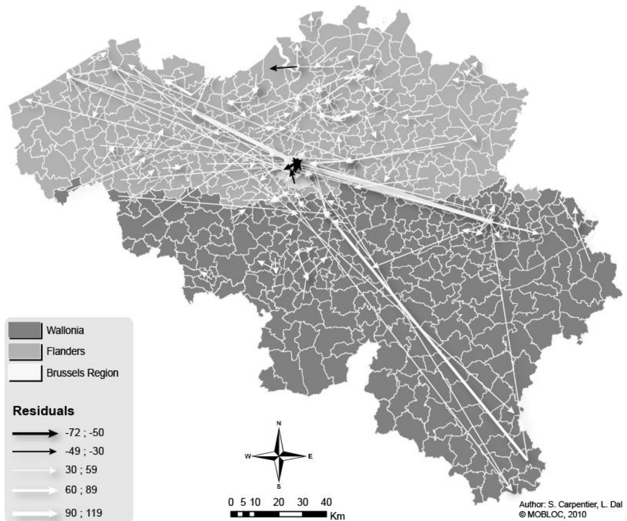
Figure 11: Inter-municipalities residuals
