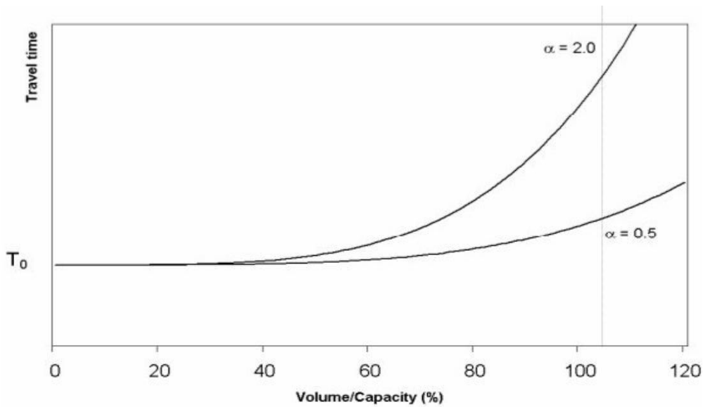
Figure 4: BPR curve (Bureau of Public Roads (1964))
