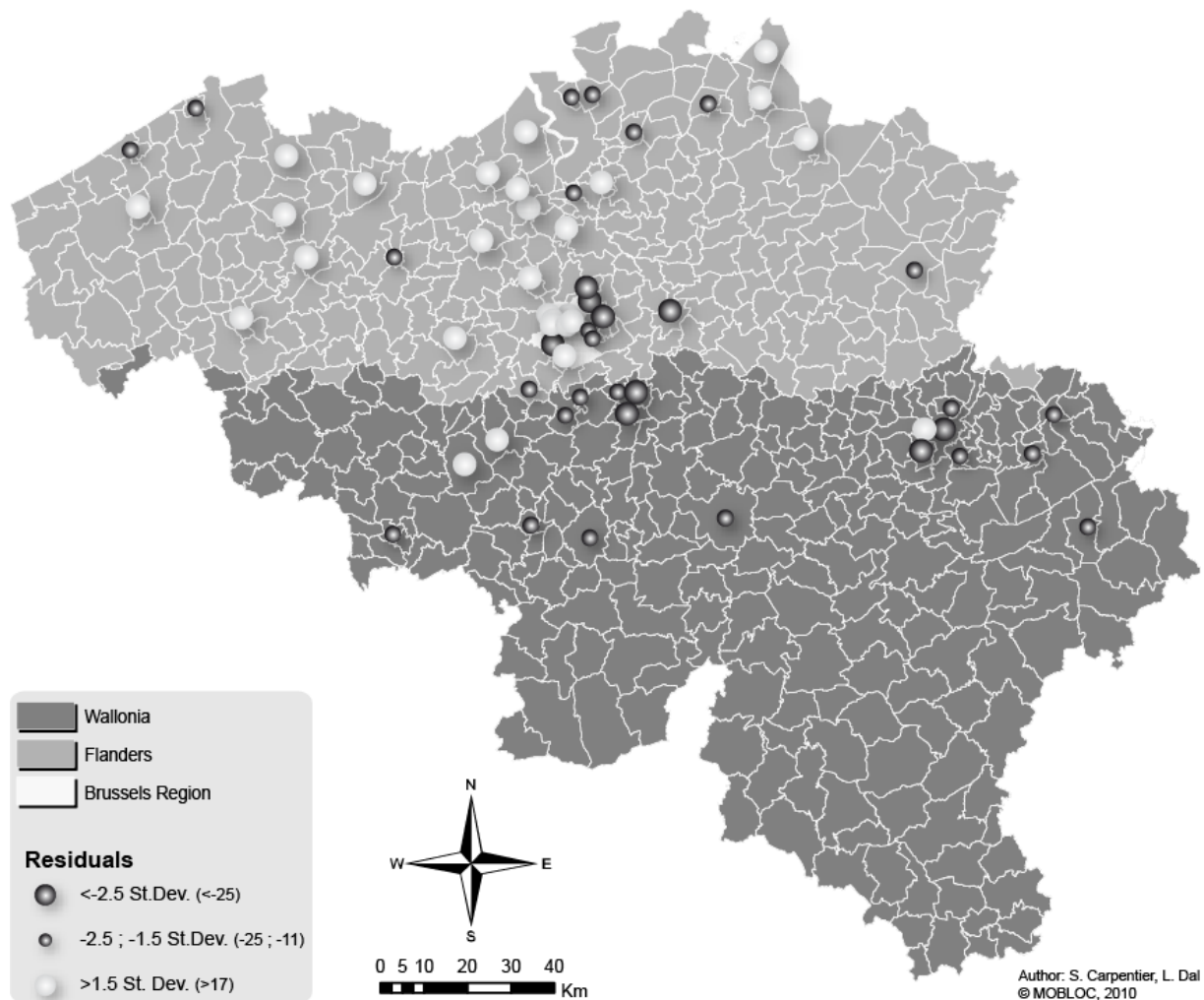
Figure 12: Intra-municipalities residuals
