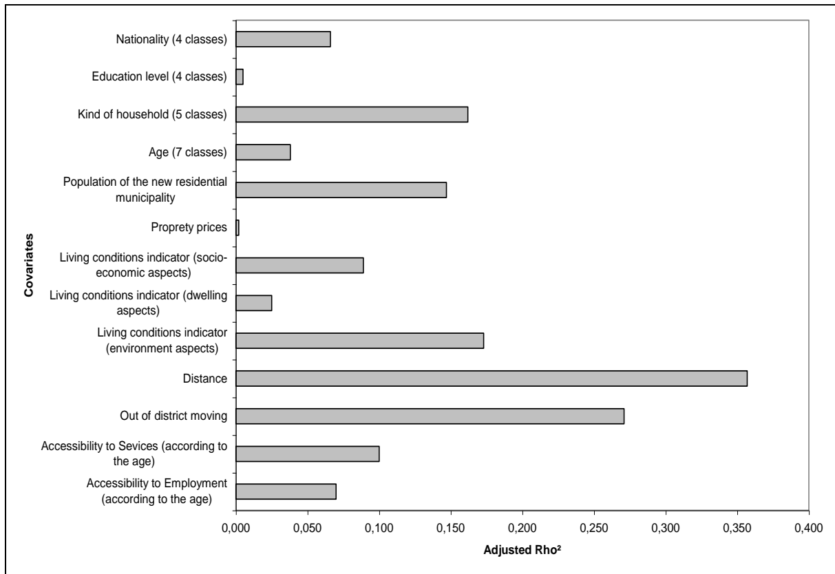
Figure 15: Adjusted Rho 2 of each covariate taken as only explanatory variable
