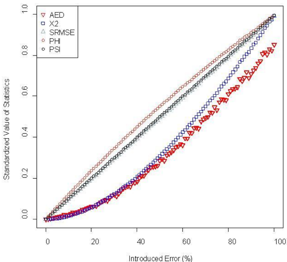
Figure 5: Error sensitivity of five Goodness-of-fit statistics
