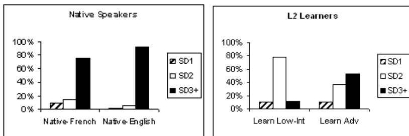
Figure 1. Overall utterance density
