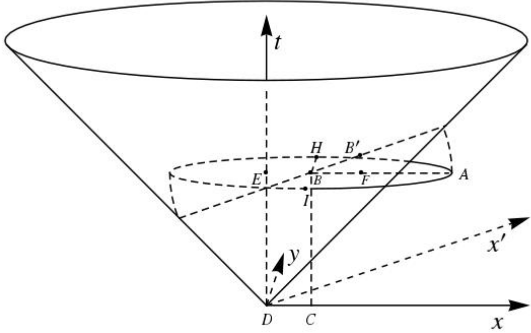
Figure 2.6: Spacetime model of Poincaré's light ellipse (1906) in a spacelike plane ( t = \text{const.} ).
