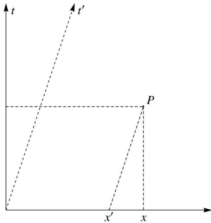
Figure 2.4: A reconstruction of Minkowski's depiction of the kinematics of Lorentz and Einstein.
