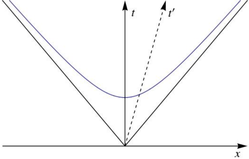
Figure 2.2: A reconstruction of Minkowski's 5 Nov. 1907 presentation of relativistic velocity space, with a pair of temporal axes, one spatial axis, a unit hyperbola and its asymptotes.
