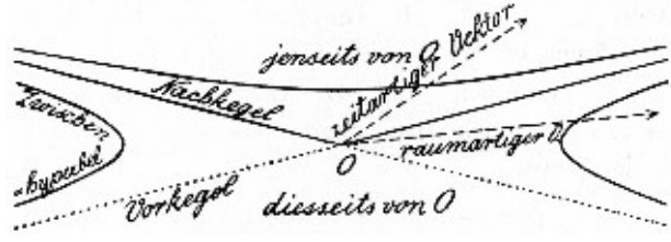
Figure 2.3: The lightcone structure of spacetime [1].
