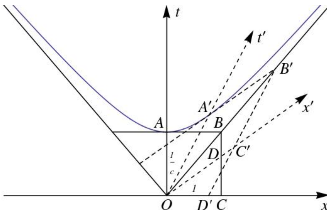
Figure 2.5: Minkowski's spacetime diagram, after [1].
