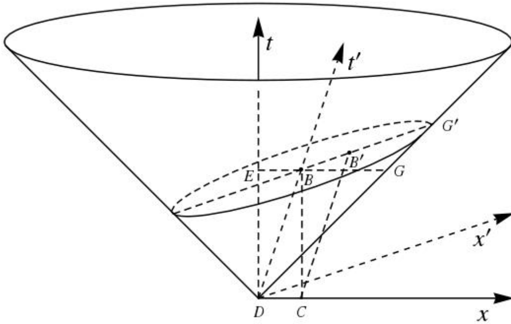
Figure 2.7: Spacetime model of Poincaré's light ellipse (1909) in a spacelike plane ( t' = \text{const.} ).
