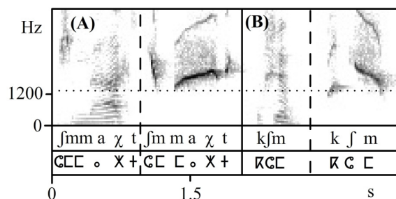
Figure 3: Spoken and whistled forms of (A) [ʃm.mart] and (B) [k.ʃm] (where . indicates syllable boundary).
