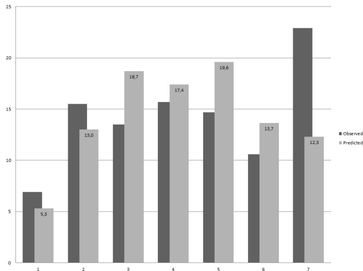
Figure 2: Distribution of the number of votes per ballot
