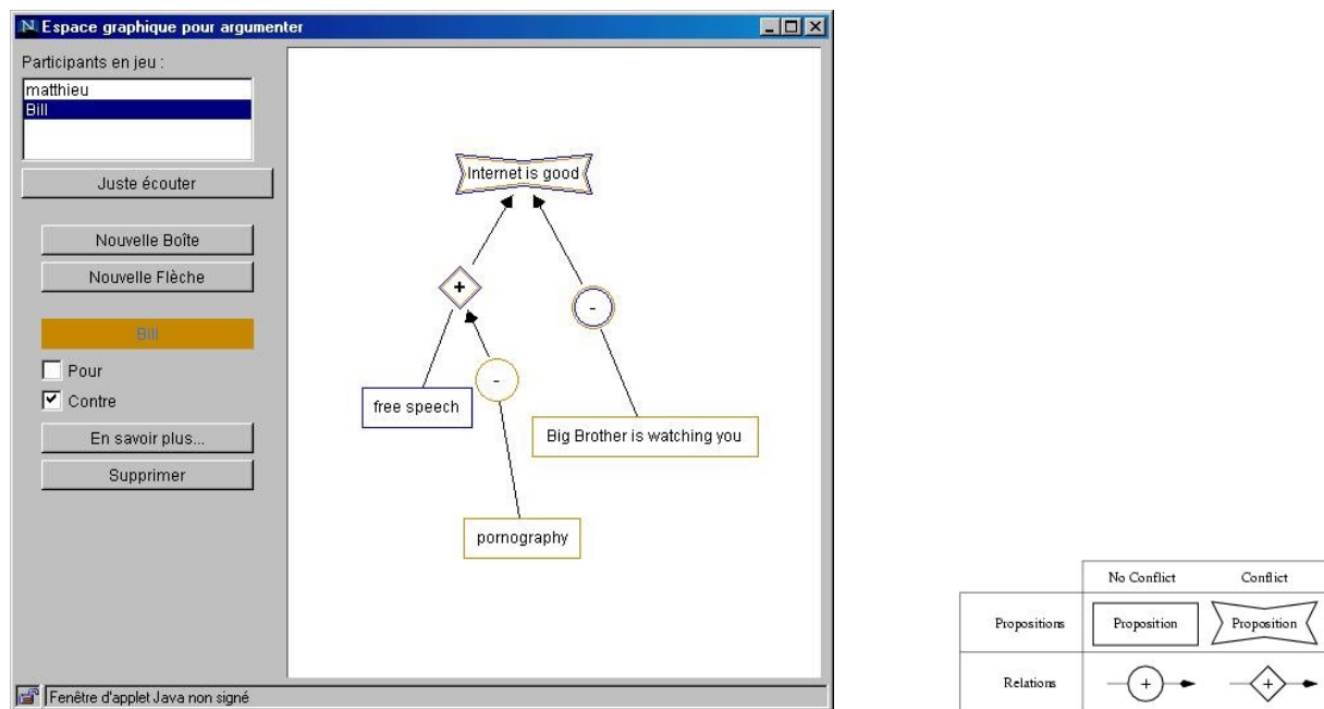
FIG. 1 – The Java Interface for Graphical Argumentation in DREW
