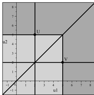
(c) Antileximax
