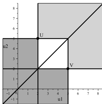
(a) Suppes
