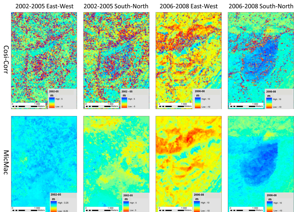
Figure 4. Maps of east-west and south-north displacements measured by Cosi-Corr and MicMac. The shift between 2002 and 2005 is close to 0 m in both directions. The EW shift between 2006 and 2008 is strongly correlated to the topography (see Figure 1B) and cannot be interpreted as displacement. The south-north shift between 2006 and 2008 is clearly detected by the two methods. It reaches around 10 m toward the north. The results produced by Cosi-Corr are noisier than those produced by MicMac as already noticed by [18].
