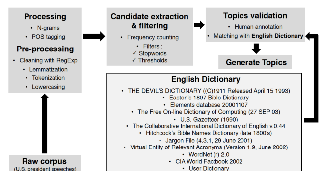
Figure 1: Data processing structure. Framework for topic acquisition from corpus data.
