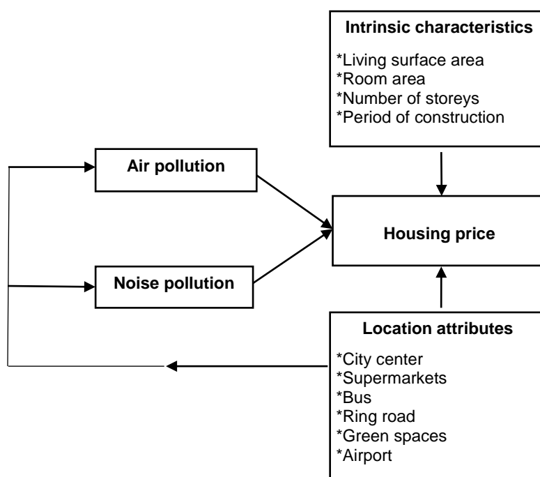
Fig.2. The hypothesized relationships between the variables
