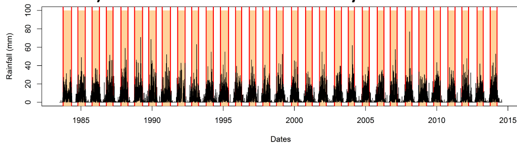
Figure 2. Illustration of the computation of the rainy season temporal metrics based on the method proposed by Liebmann et al. [33]. It includes: (A) a one-year daily rainfall time series for a given pixel; (B) the corresponding anomalous accumulation time series with identified onset and demise dates; (C) the entire (31-year) daily rainfall time series for a given pixel and its corresponding onset and demise dates.
