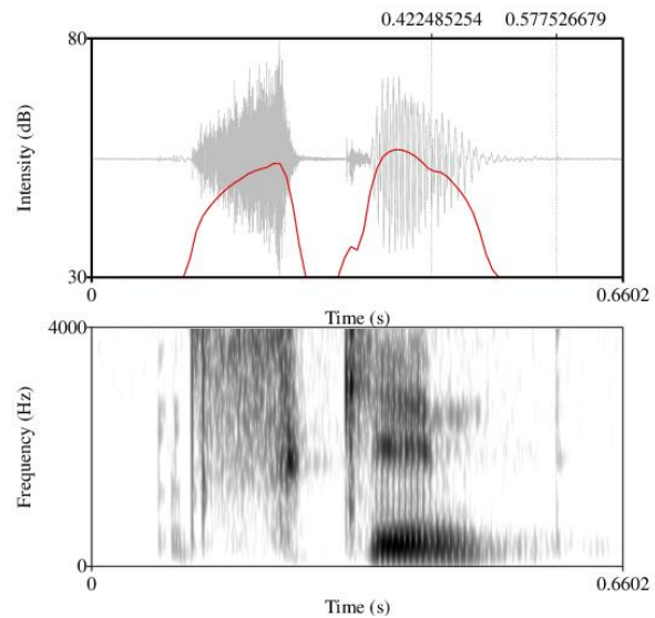
Figure 7 skin [skʰinʔ]
