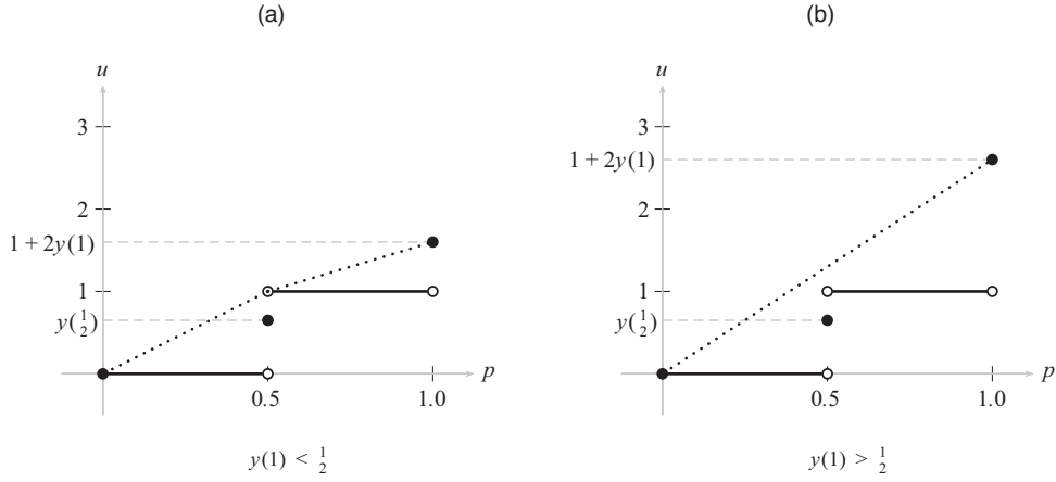
Figure 1. Concavification in Example 2. u(y(p); p) in solid lines and \text{cav}_p u(y(p); p) in dotted lines.
