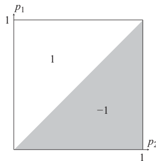
Figure 2. Payoff of designer 1 in Example 3 as a function of the agent's beliefs (p_1, p_2) .
