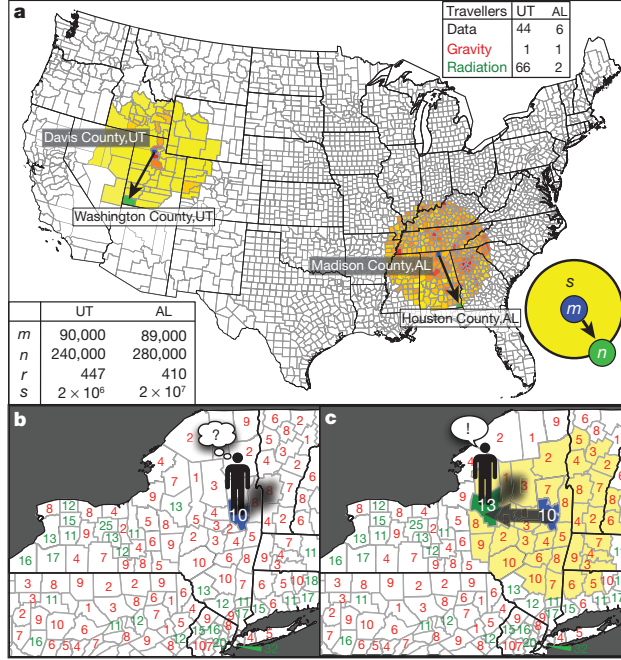
Fig. 26: Schematic of the the radiation model. (a) Commuting flows in two pairs of counties, one in Utah (UT) and the other in Alabama (AL), with similar origin ( m , blue) and destination ( n , green) populations and comparable distance r between them (see bottom left table). Number of travelers in the data, as predicted by the gravity model and finally for the radiation model shown as upper right inset. The definition of the radiation model: (b) An individual (e.g. living in Saratoga County, NY) applies for jobs in all counties and collects potential employment offers. The number of job opportunities in each county is chosen to be proportional to the resident population. Each offers attractiveness (benefit) is represented by a random variable with distribution p(z) , the numbers placed in each county representing the best offer among the jobs in that area. Each county is marked in green (red) if its best offer is better (lower) than the best offer in the home county. (c) An individual accepts the closest job that offers better benefits than his home county. Figure from [42].
