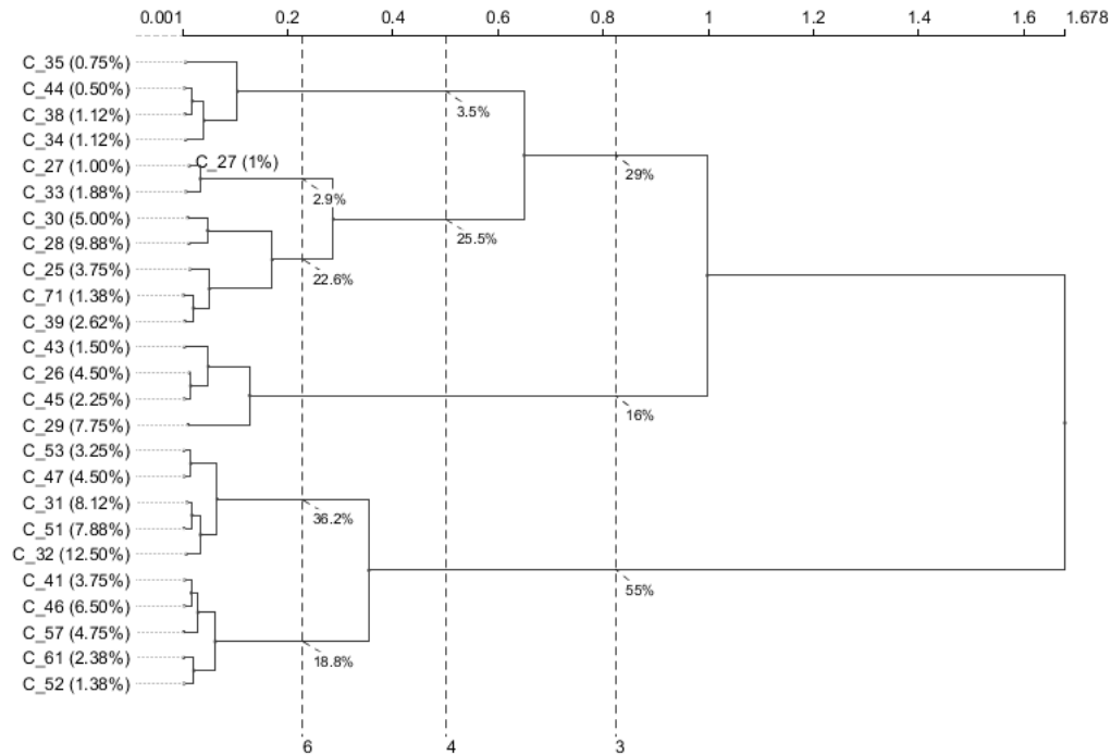
Figure 2 Dendrogram, Agglomerative Hierarchical Clustering based on the Ward criterion for the subset of 800 routes
