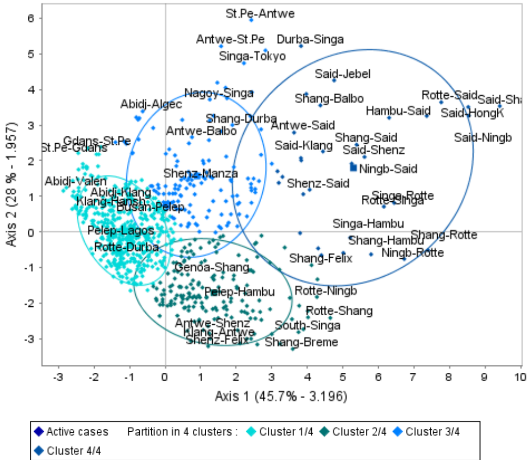
Figure 3 Graphical representation of the four clusters on the first two PCA axes
