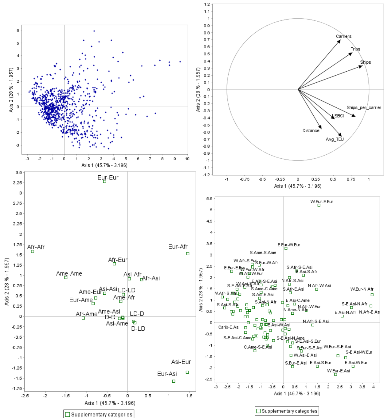
Figure 1: On the upper-left corner: the factorial map of individuals; On the upper- right corner: representation of the active continuous variables; On the lower-left corner: representation of the supplementary categorical variables related to the Trade Direction and the Trade between continents; On the lower-right corner: representation of the supplementary categorical variables related to trade between regions.
