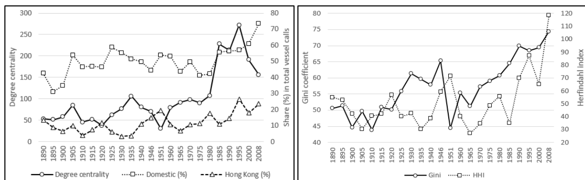
Figure 2. Maritime connectivity of mainland Chinese ports, 1890-2008
