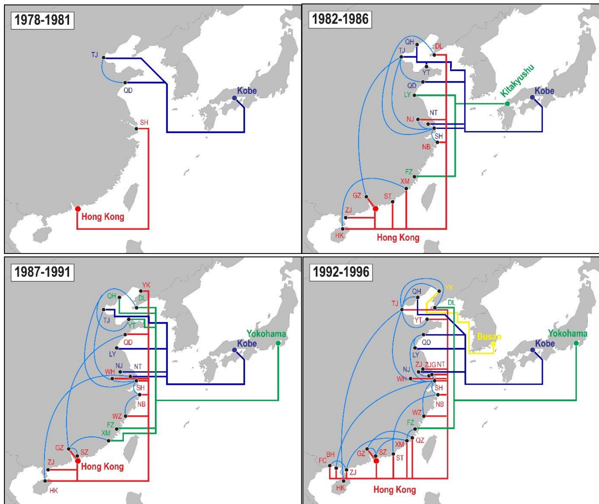
Figure 10. Dominant linkages among Chinese ports and with Northeast Asian ports, 1978-2016
