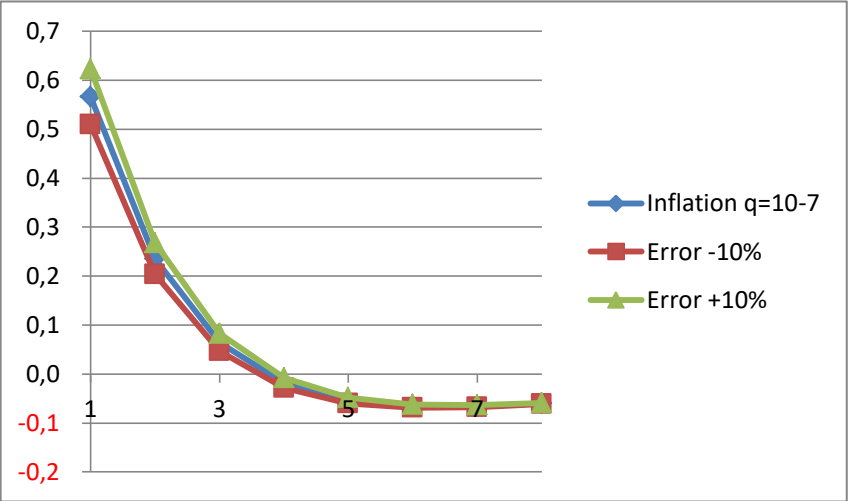
Figure 8 Impulse response of inflation: q=10^{-7} and out of equilibrium path +/- 10% error.
