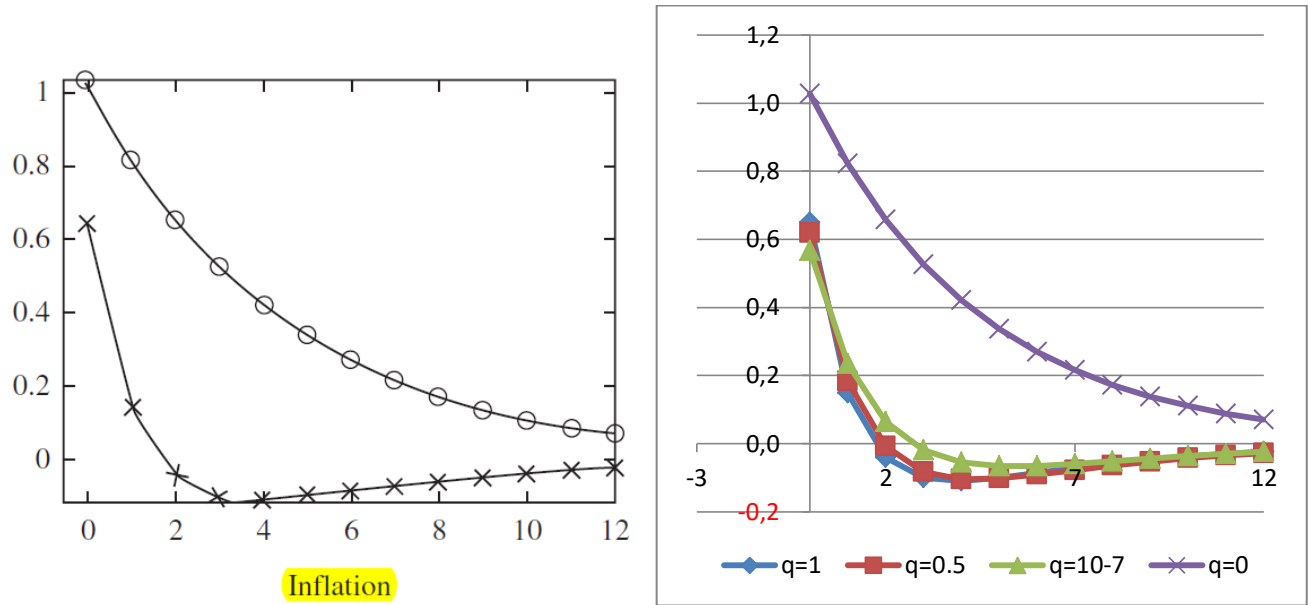
Figure 8 Impulse response of inflation: q=10^{-7} and out of equilibrium path +/- 10% error.
