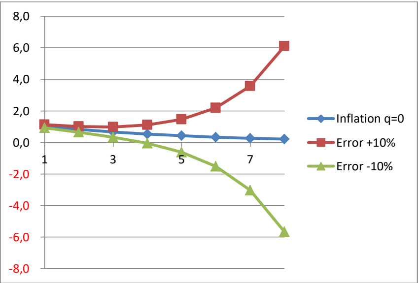
Figure 9. Impulse response of inflation: q=0 and out of equilibrium path +/- 10% error.
