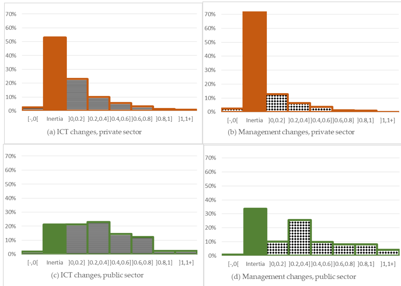
Figure 1. Distribution of ICT and management changes in the populations of private and public organizations. Data source: COI 2006/INSEE-DARES-CEE, COIFP 2006/DGAFP-DARES-CEE. Coverage: Productive units of 20 or more employees in the private sector and of 10 or more employees in the public sector. Weighted data. Note: The unit of the horizontal axis expresses the intensity of change in the metric of the MCA performed in 2006 for each type of change.
