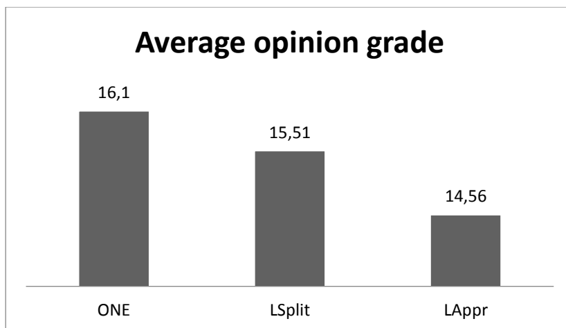
FIG. 2 – Average opinion grade of supported lists under the different voting rule
