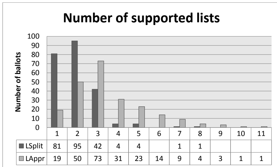
FIG. 1 – Distribution of the number of supported lists under the LSplit and LAppr rules
