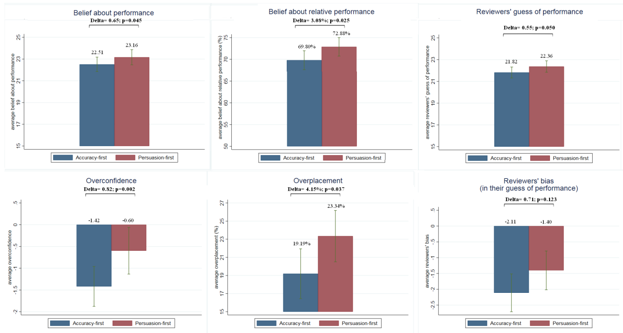
Figure 3: A summary of our main variables of interest comparing Accuracy-first treatment (in blue bars) and Persuasion-first treatment (in red bars) with mean values, treatment differences and p-values (from two-sided Mann-Whitney rank-sum tests) indicated on top. All information conditions in Study 1 are pooled together.
