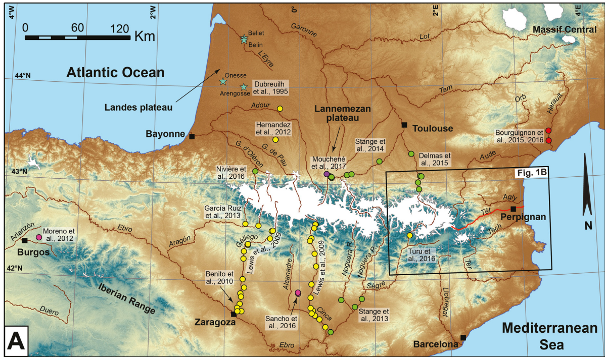
● ESR ● OSL ● TCN profiles ● TCN exposure ● 39 Ar/ 40 Ar ★ Biostratigraphic ages previously published Late Pleistocene ice extent after Calvet et al., 2011. River network after HYDROSHEDS (Lehner & Grill, 2013).
