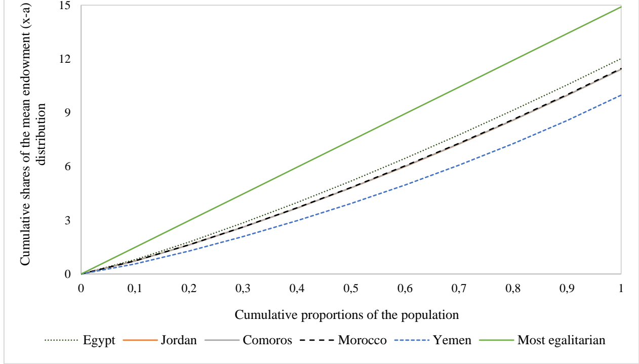
Figure 5: Generalized Lorenz curves of the lower tail BMI distribution in five Arab Countries ( a = 10 and m = 24.9 )
