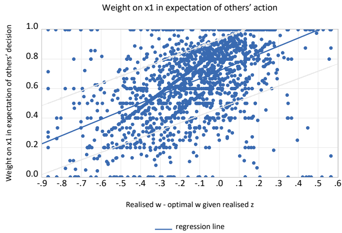
(b) Weight assigned to x_1 in the expectation of others' decision as a function of difference between realised \omega and optimal \omega given realised z in treatment B
